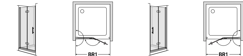
View, hinged left
