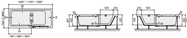
Top view 608.301100 / 608.300100 / 608.302100 View 608.301100 / 608.300100 / 608.302100 View 608.301200 / 608.300200 / 608.302200
