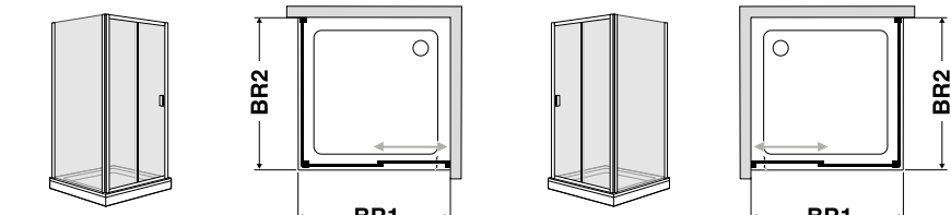
View, side panel left Top view, side panel left View, side panel right Top view, side panel right
