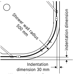
Installation dimension
