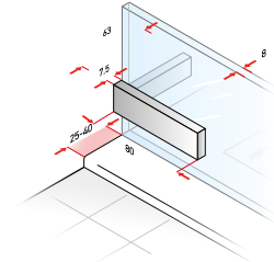
Fixed panel and side panel
