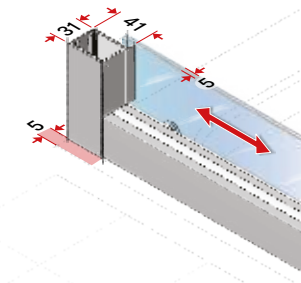
Door parts closure
