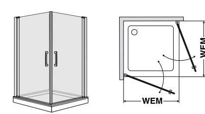
View Top view
