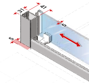
Door parts closure internal
