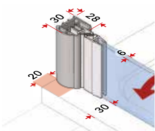
Door parts closure
