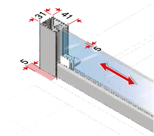
Door parts closure external
