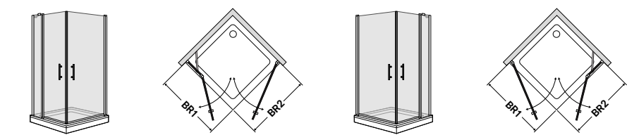
View, fixed panel left Top view, fixed panel left View, fixed panel right Top view, fixed panel right
