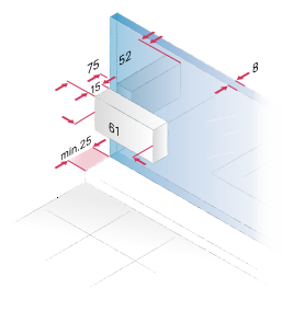
Fixed panel and side panel
