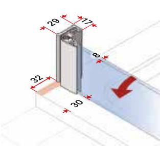
Door parts closure
