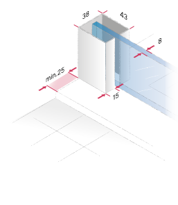
Fixed panel and side panel with wall profile
