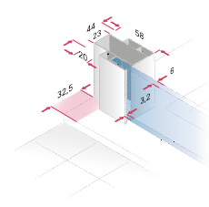
Fixed panel and side panel
