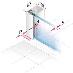
Fixed panel and side panel
