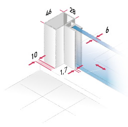
Door panel closing side
